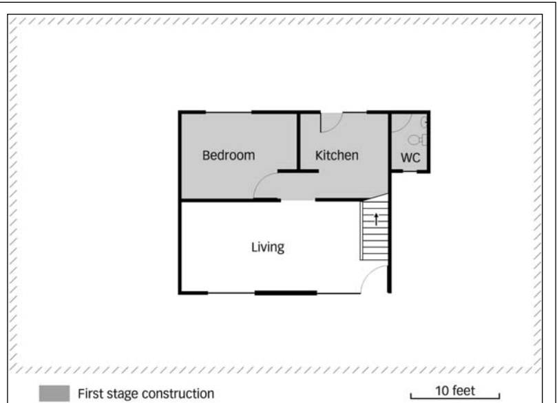
FIGURE 3 Part of the plans for one of three house types being built in the first phase of Dandaniyawatta's upgrading
